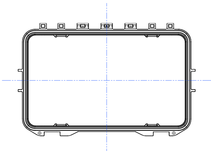
Vista Interna Coperchio Lid Inner View
