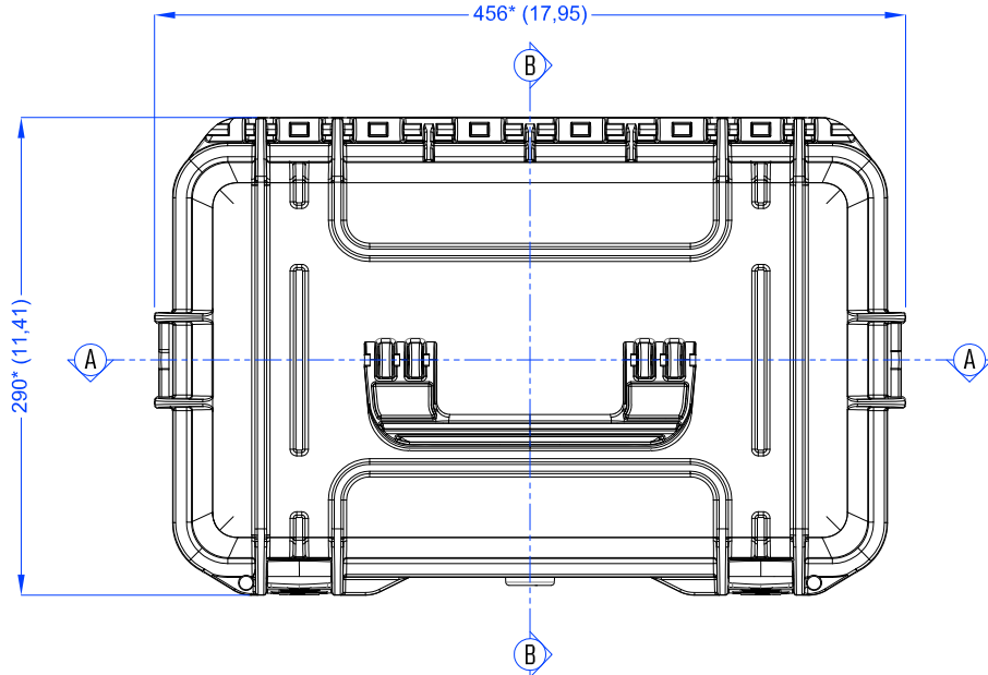
Vista Coperchio Lid View
